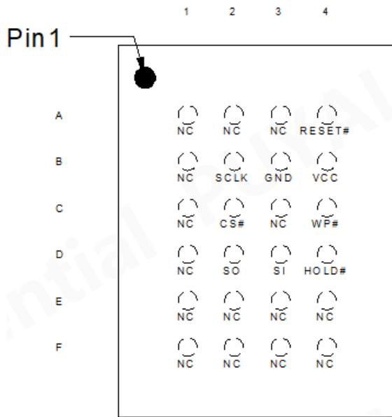
24-Ball TFBGA (4x6 Array) -TB
