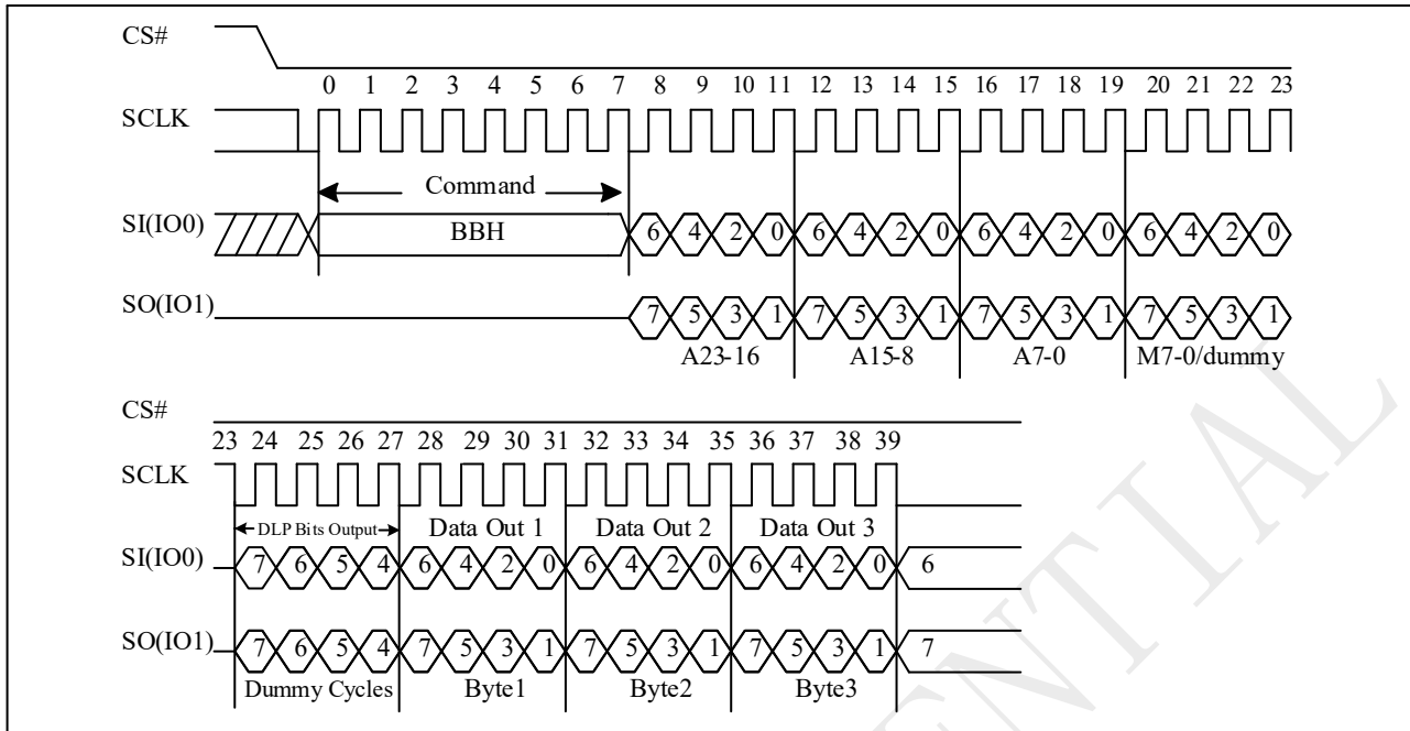
Figure 10-30d 2IO Read (Choose 8 dummy) with DLP bits output Sequence (SPI)
