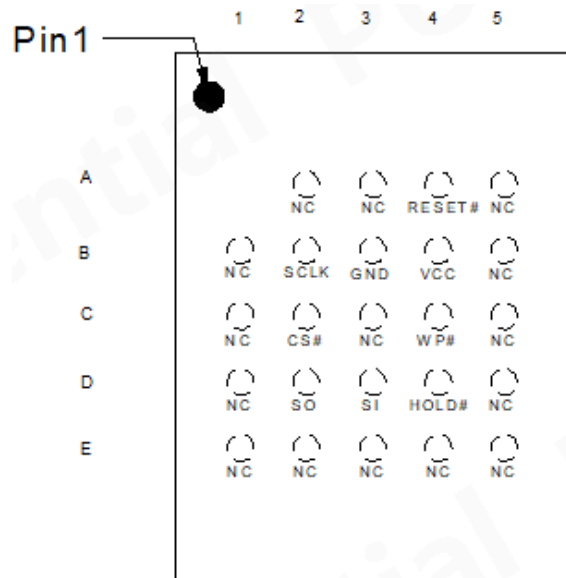
24-Ball TFBGA (5x5 Array) -TF
