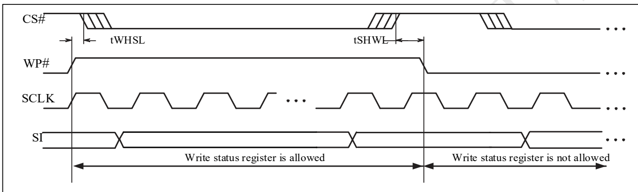
Figure 5-7 WP Timing
