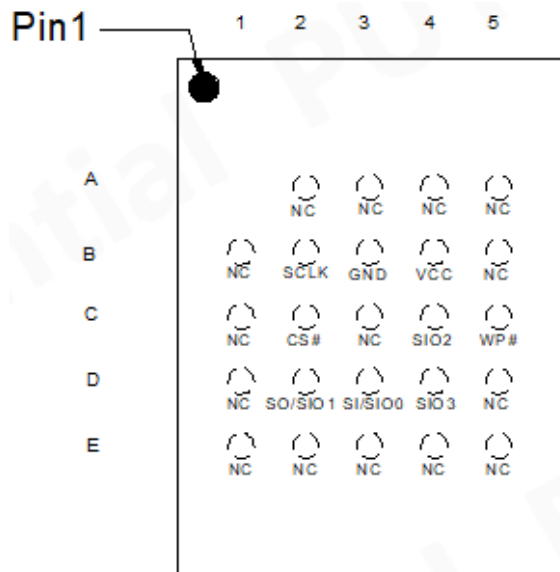
24-Ball TFBGA (5x5 Array) -TN
