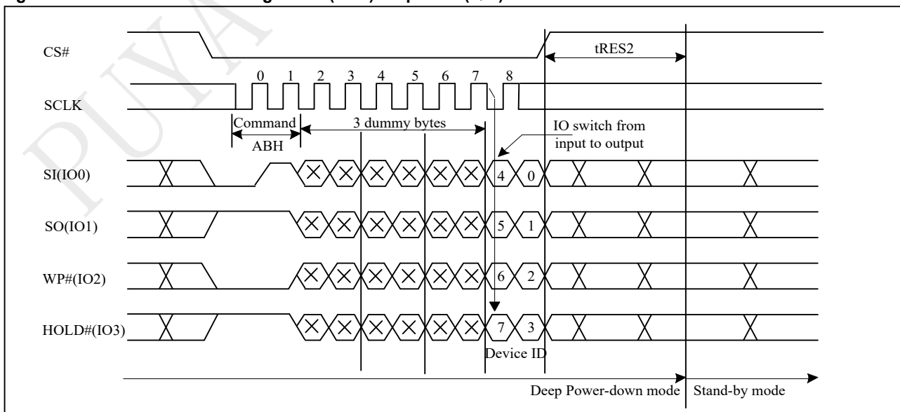
Figure 10-50a Read Electronic Signature (RES) Sequence (QPI)
